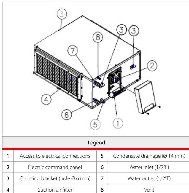
Figure 3 - Connections
