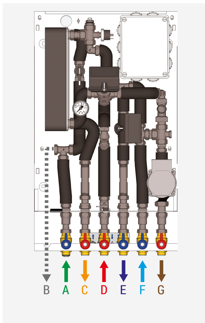
Installation example: GE551Y134 template + GE556Y406 HIU
